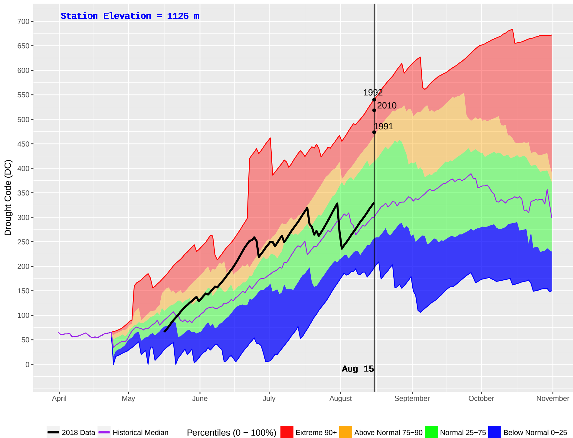
BLACKPINE (148) : Historical (1980–2016) and Current (2018) Daily Drought Code (DC)
