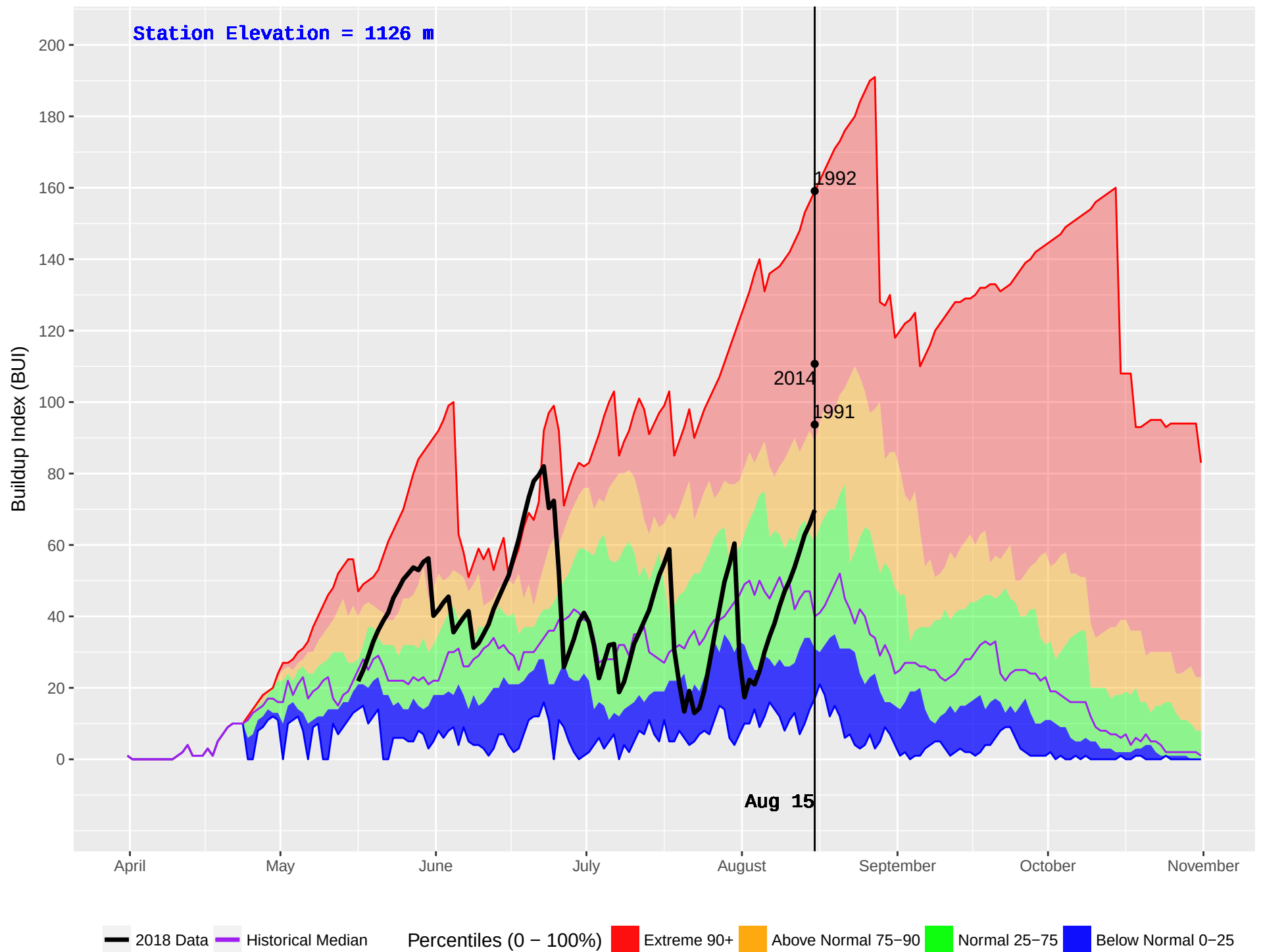
BLACKPINE (148) : Historical (1980–2016) and Current (2018) Daily Buildup Index (BUI)
