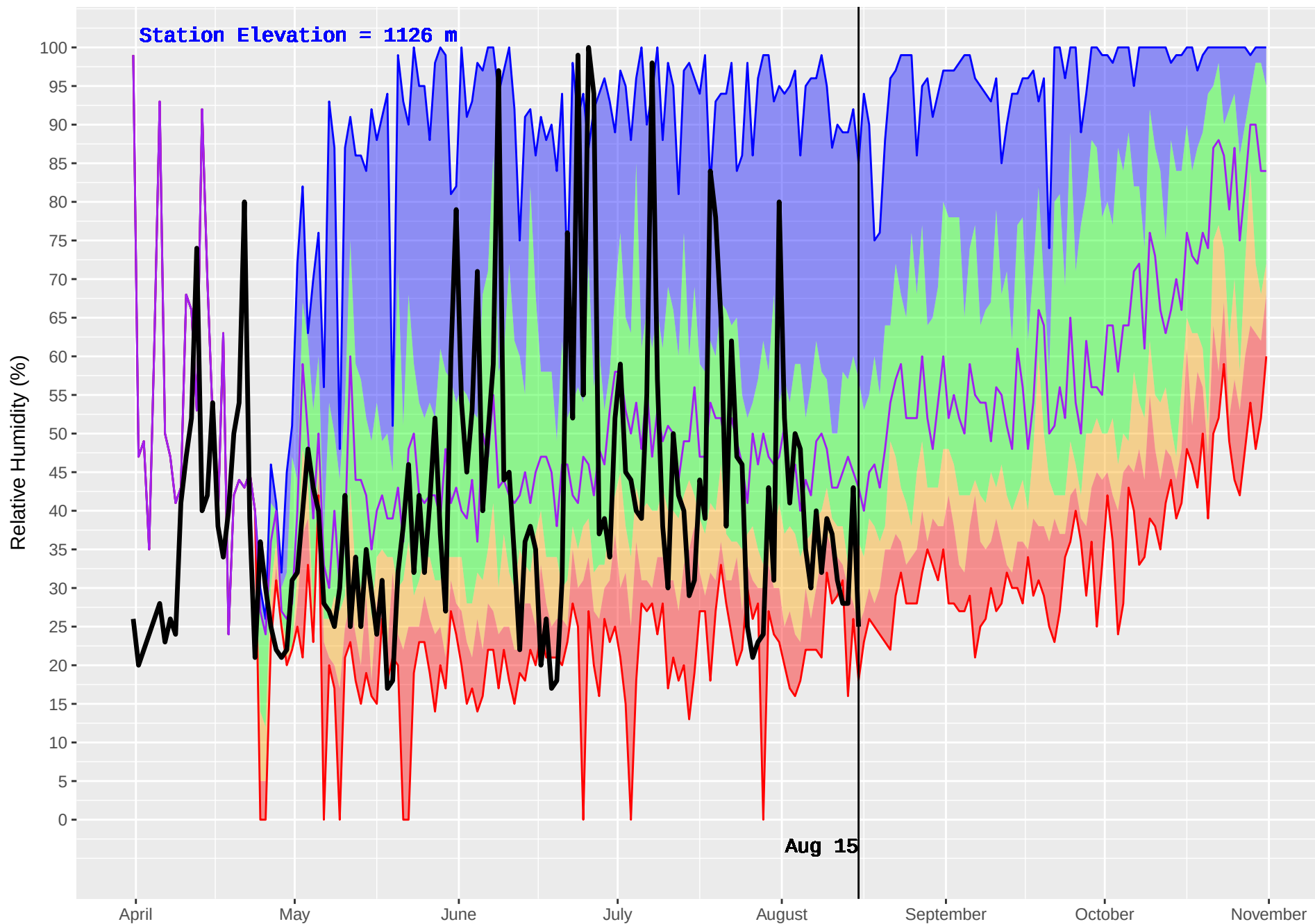
BLACKPINE (148) : Historical (1980–2016) and Current (2018) Daily Relative Humidity
