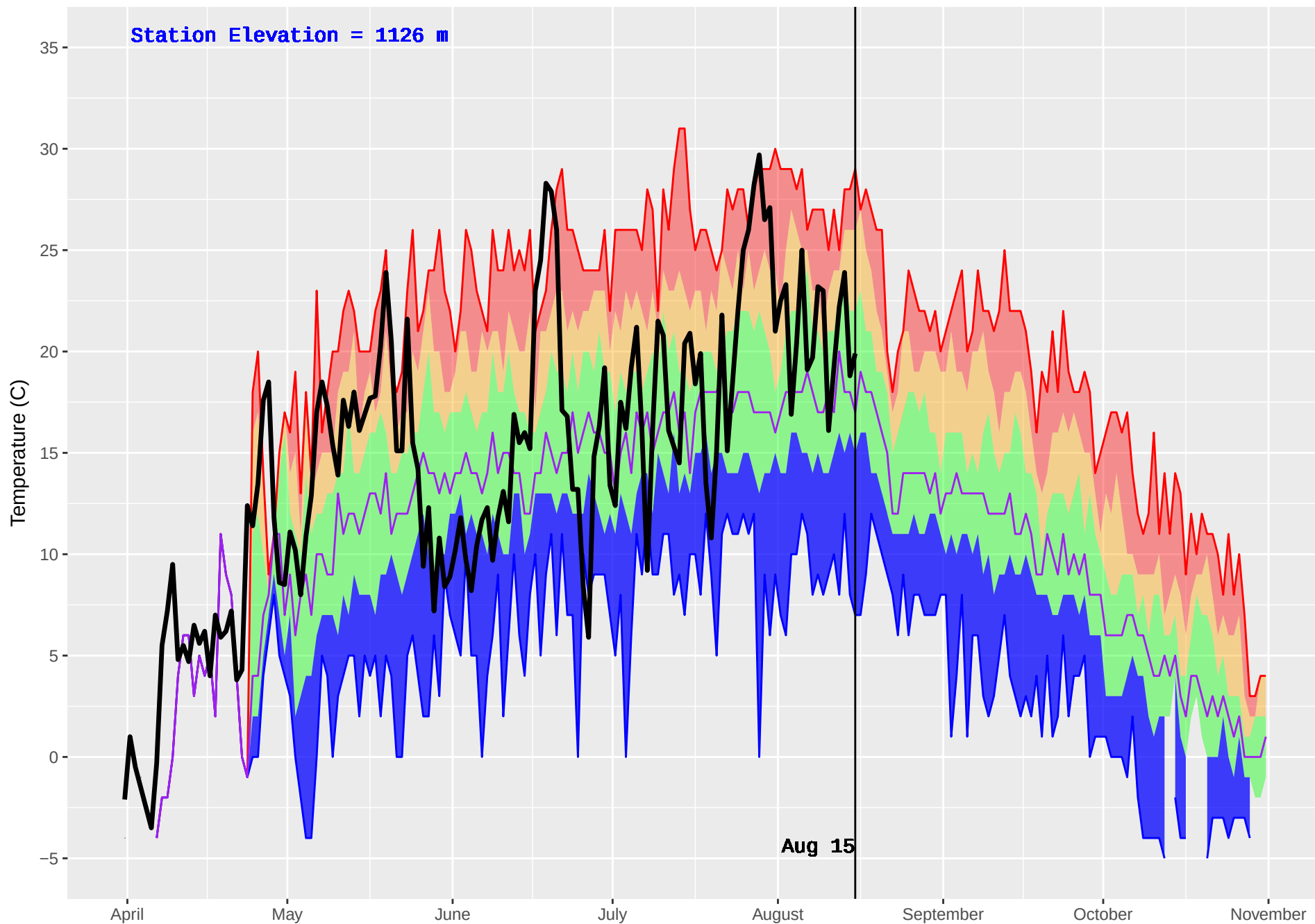
BLACKPINE (148) : Historical (1980–2016) and Current (2018) Daily Temperature
