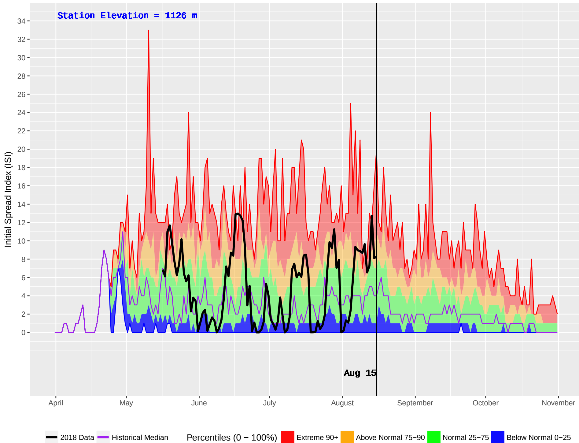
BLACKPINE (148) : Historical (1980–2016) and Current (2018) Daily Initial Spread Index (ISI)
