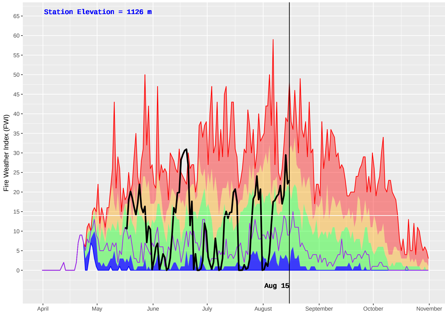
BLACKPINE (148) : Historical (1980–2016) and Current (2018) Daily Fire Weather Index (FWI)
