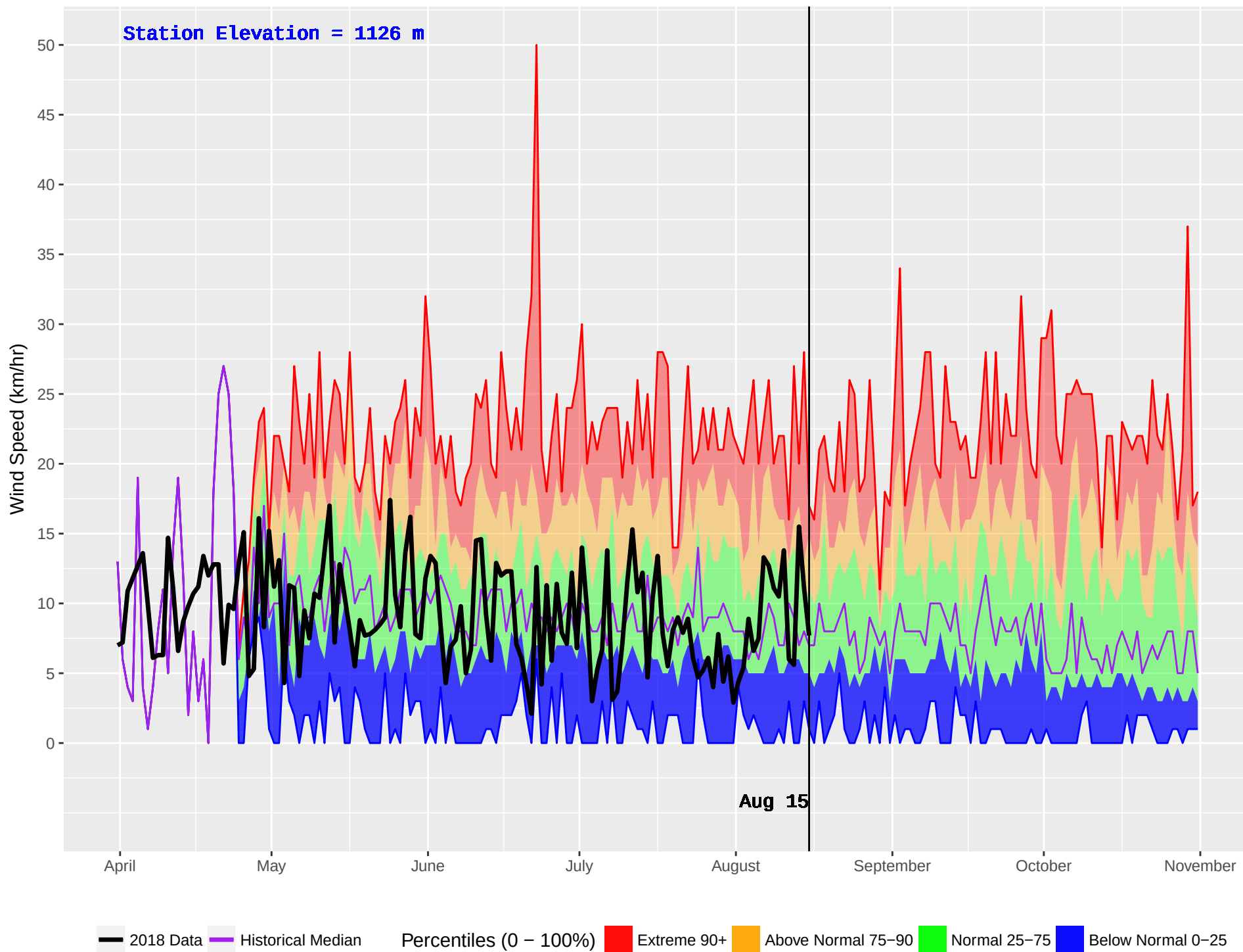
BLACKPINE (148) : Historical (1980–2016) and Current (2018) Daily Wind Speed
